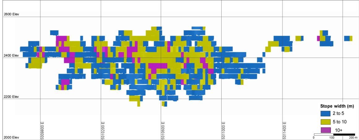
Long Section of Stope Width Gigante
